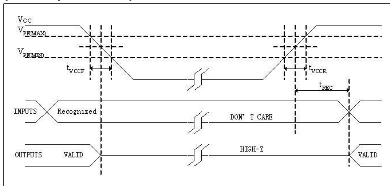
Figure 1. Power-Up/Power-Down Timing
